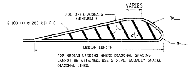
MEDIANS OVER 1.2 m (4') WIDE
