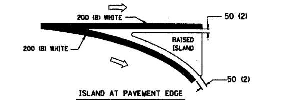
TYPICAL ISLAND MARKING
