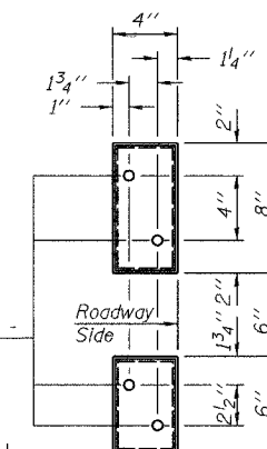
VIEW E-E
