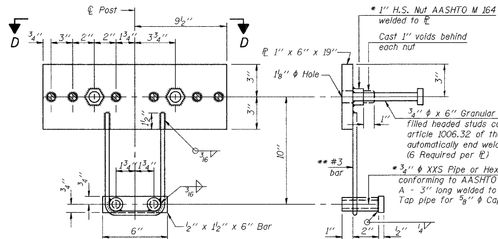
ANCHOR DEVICE
