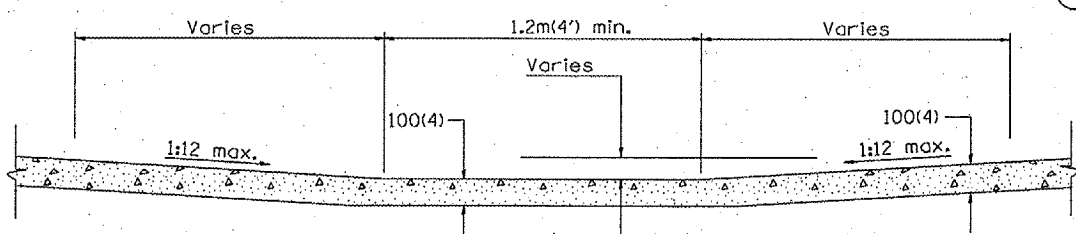
SEC. D-D
