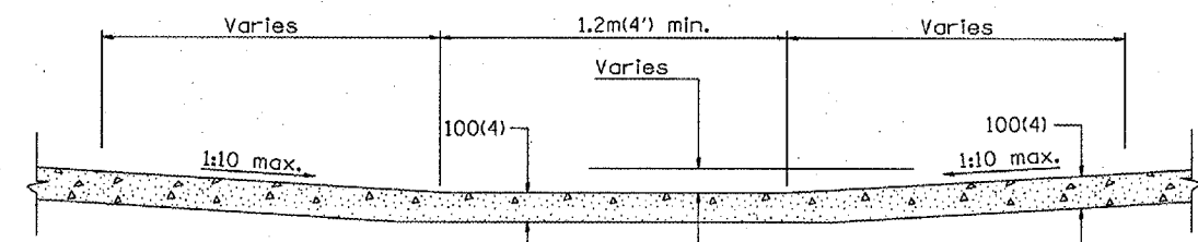
SEC. B-B
