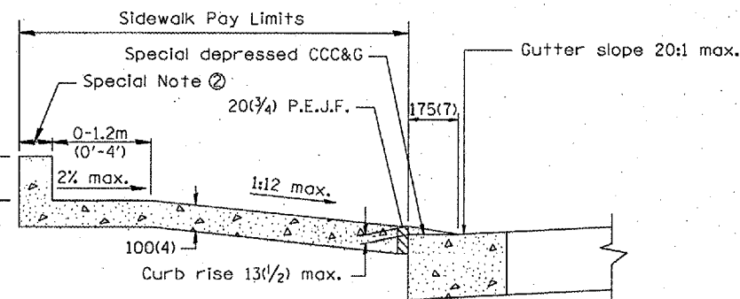
SEC. C-C
