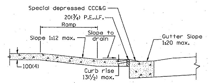
SEC. G-G
