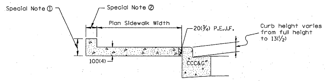
SEC. F-F
