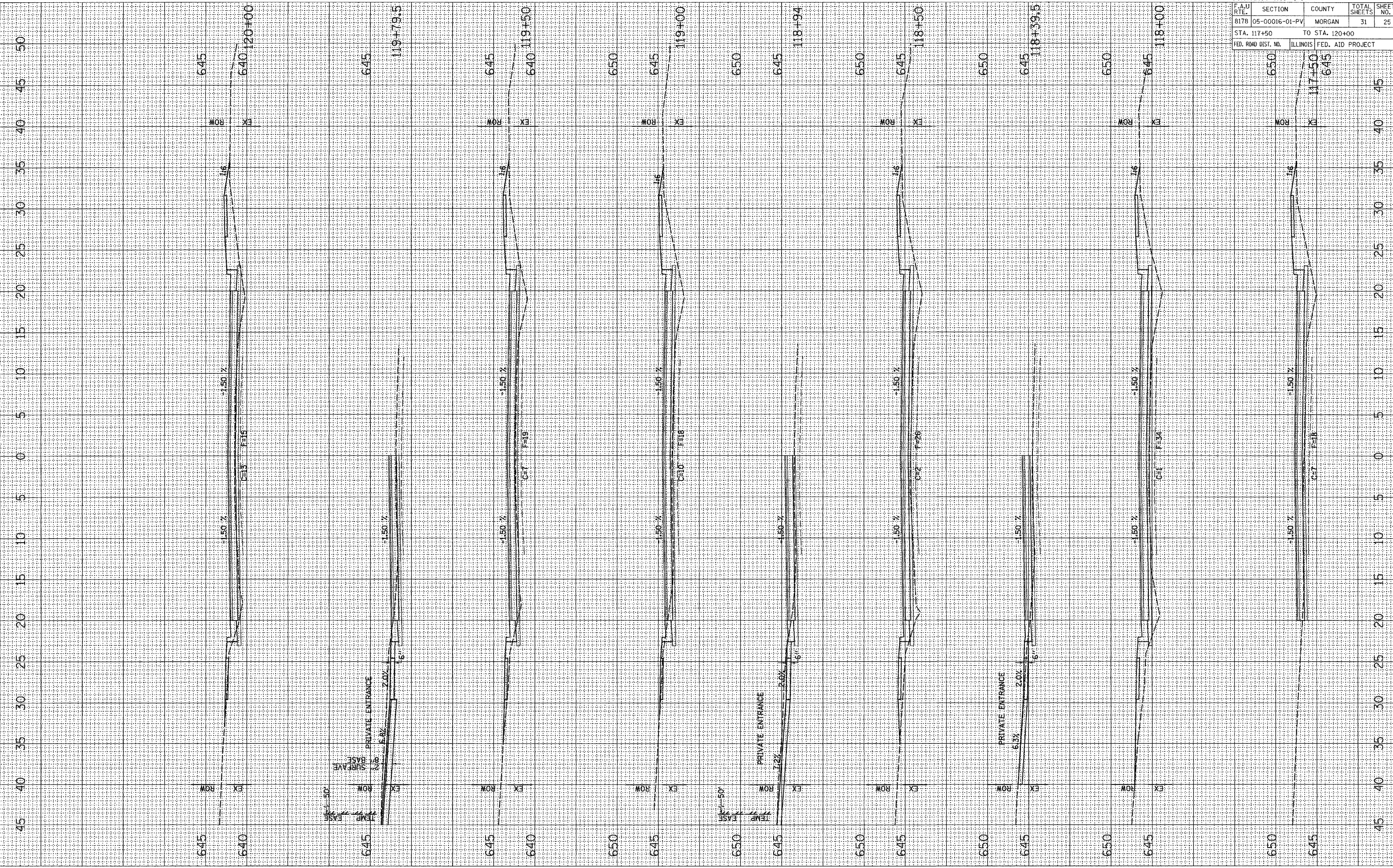
WEST VANDALIA ROAD, CROSS SECTIONS, STA 117+50 TO STA 120+00
