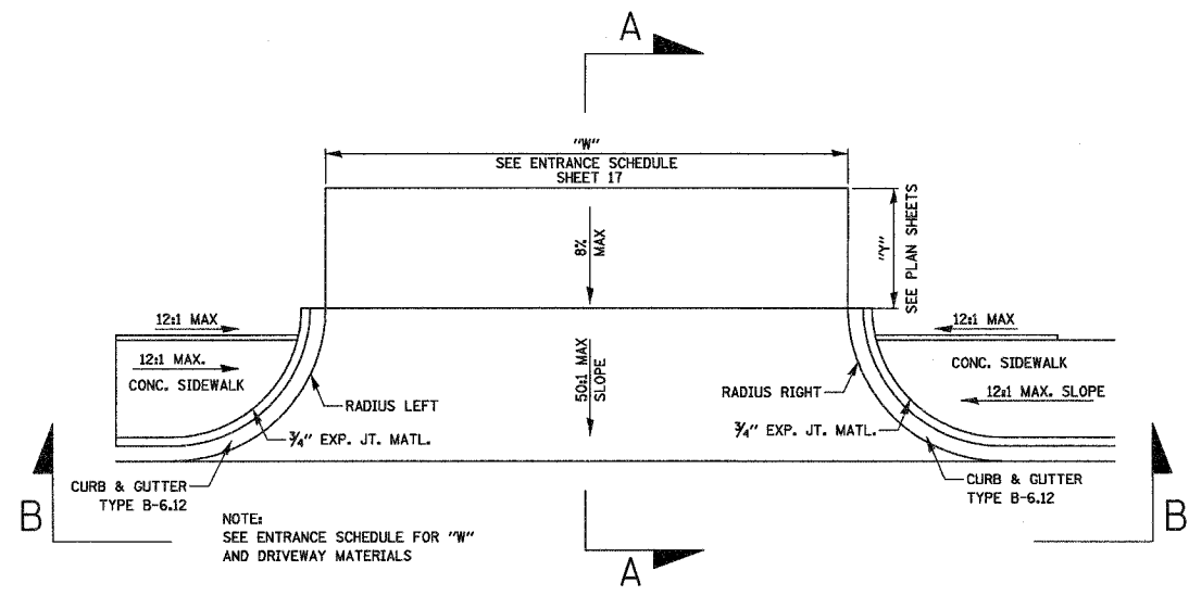
DRIVEWAY ENTRANCE DETAIL N.T.S.
