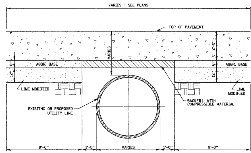
TYPICAL PROTECTION OF UTILITY LINE N.T.S.
