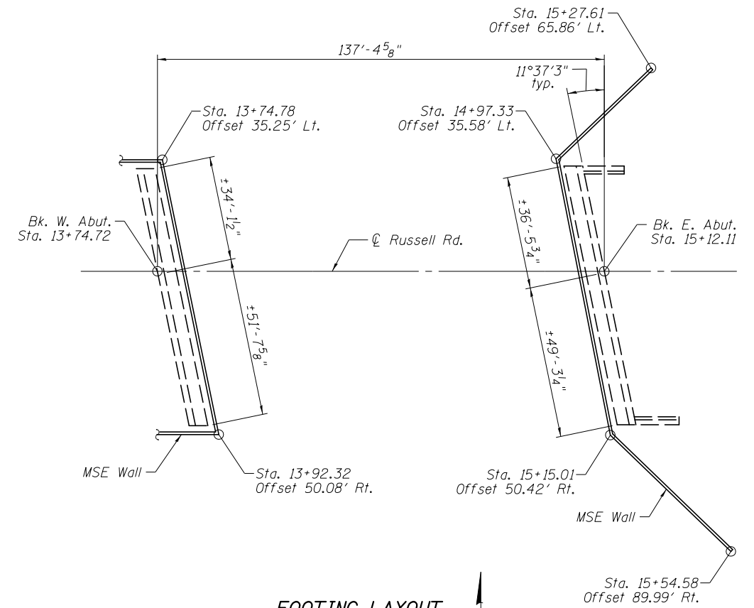
FOOTING LAYOUT
