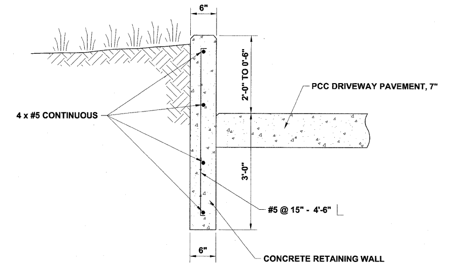
DETAIL B
