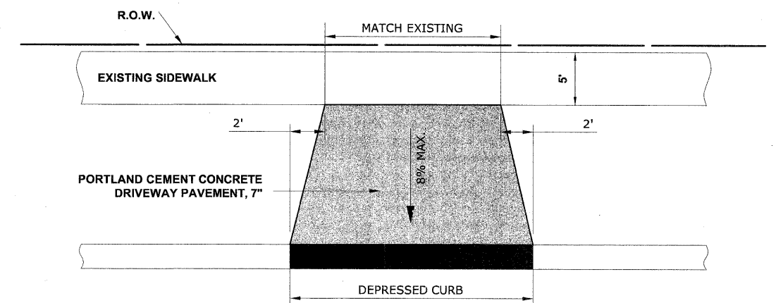
DRIVEWAY DETAIL
