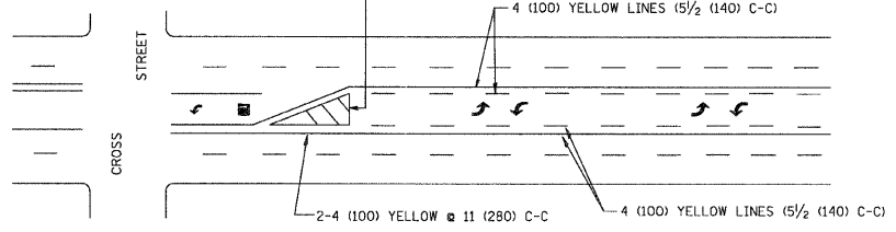
TYPICAL PAINTED MEDIAN MARKING
