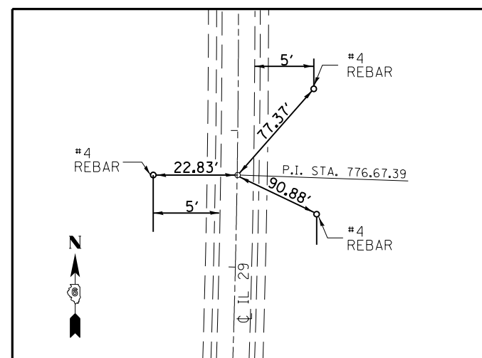
P.I. STA. 776+67.39 (SET: P.K. NAIL IN CHISELED "X")
