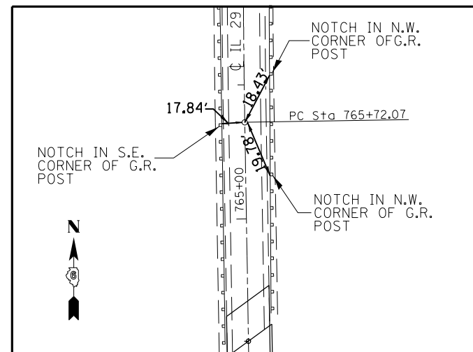
P.C. STA. 765+72.07 (FD: BRASS DISK WITH DIMPLE)
