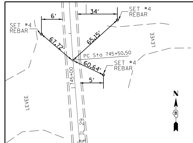
P.C. STA. 745+50.50 (FD: BRASS DISK WITH DIMPLE)
