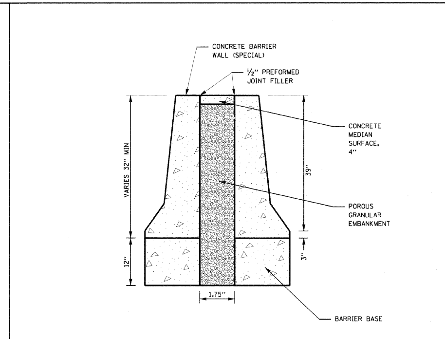
SECTION C-C CONCRETE BARRIER WALL (SPECIAL) SCALE: NONE
