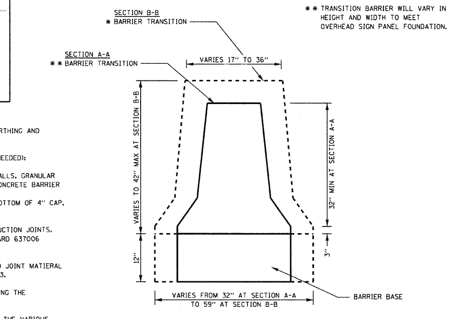
SECTION A-A SECTION B-B CONCRETE BARRIER TRANSITION SCALE: NONE
