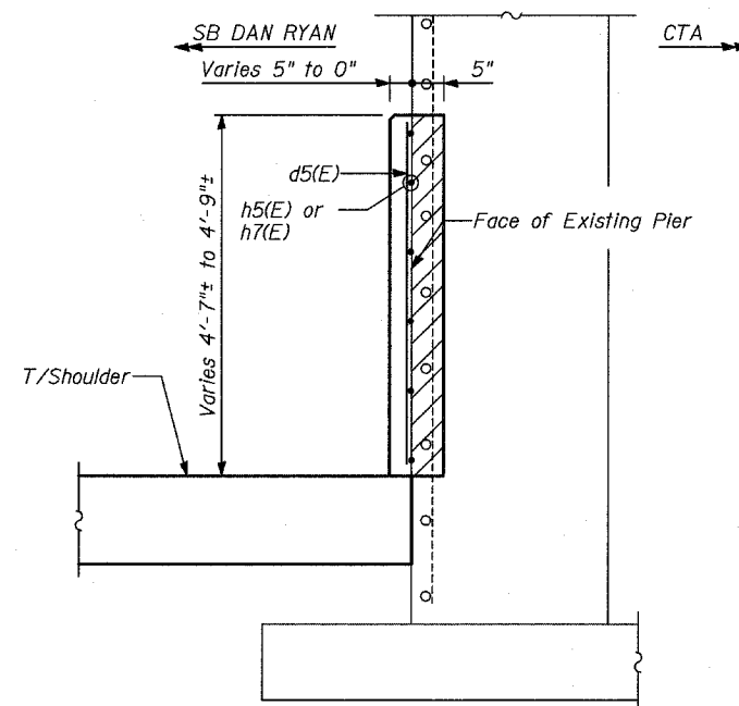
SECTION E-E
