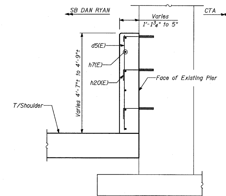
SECTION H-H
