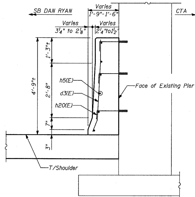
SECTION C-C
