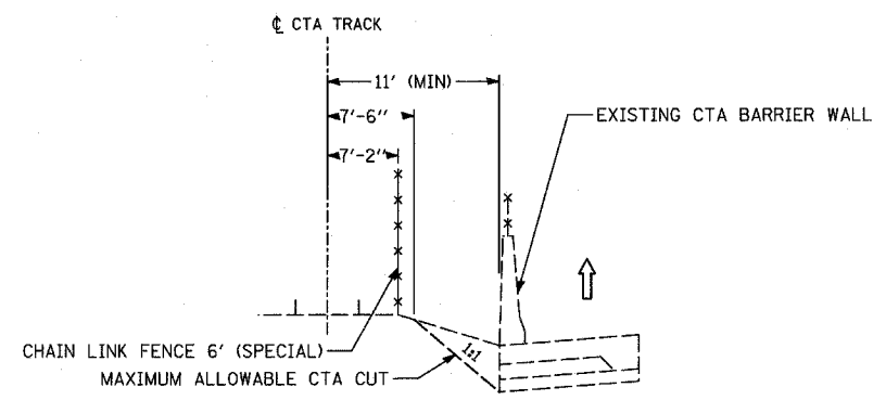
LOCATION OF CHAIN LINK FENCE 6' (SPECIAL)
