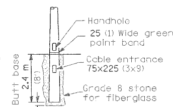
BUTT BASE
