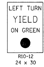
DETAIL E NOT TO SCALE
