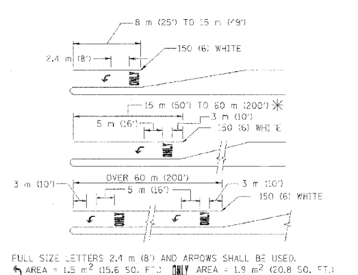
TYPICAL LEFT (OR RIGHT) TURN LANE
