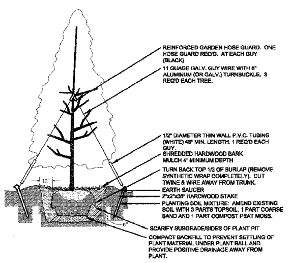
3 PLANTING DETAIL EVERGREEN NOT TO SCALE
