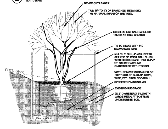
4 PLANTING DETAIL TREE ON BERM NOT TO SCALE
