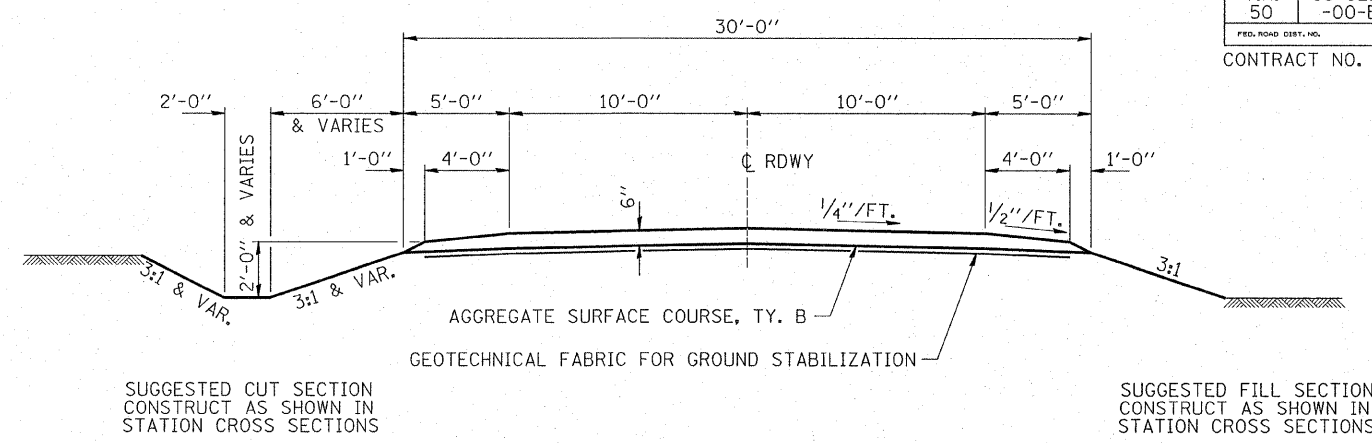
PROPOSED TYPICAL CROSS SECTION STA. 7+00 TO STA. 26+50
