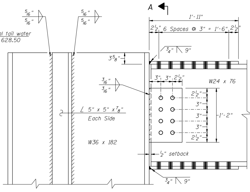
DETAIL "A" (Option 2)
