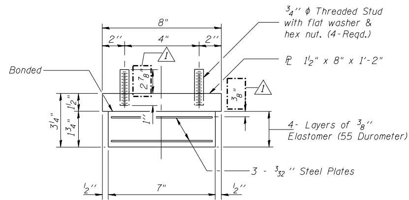
BEARING ASSEMBLY
