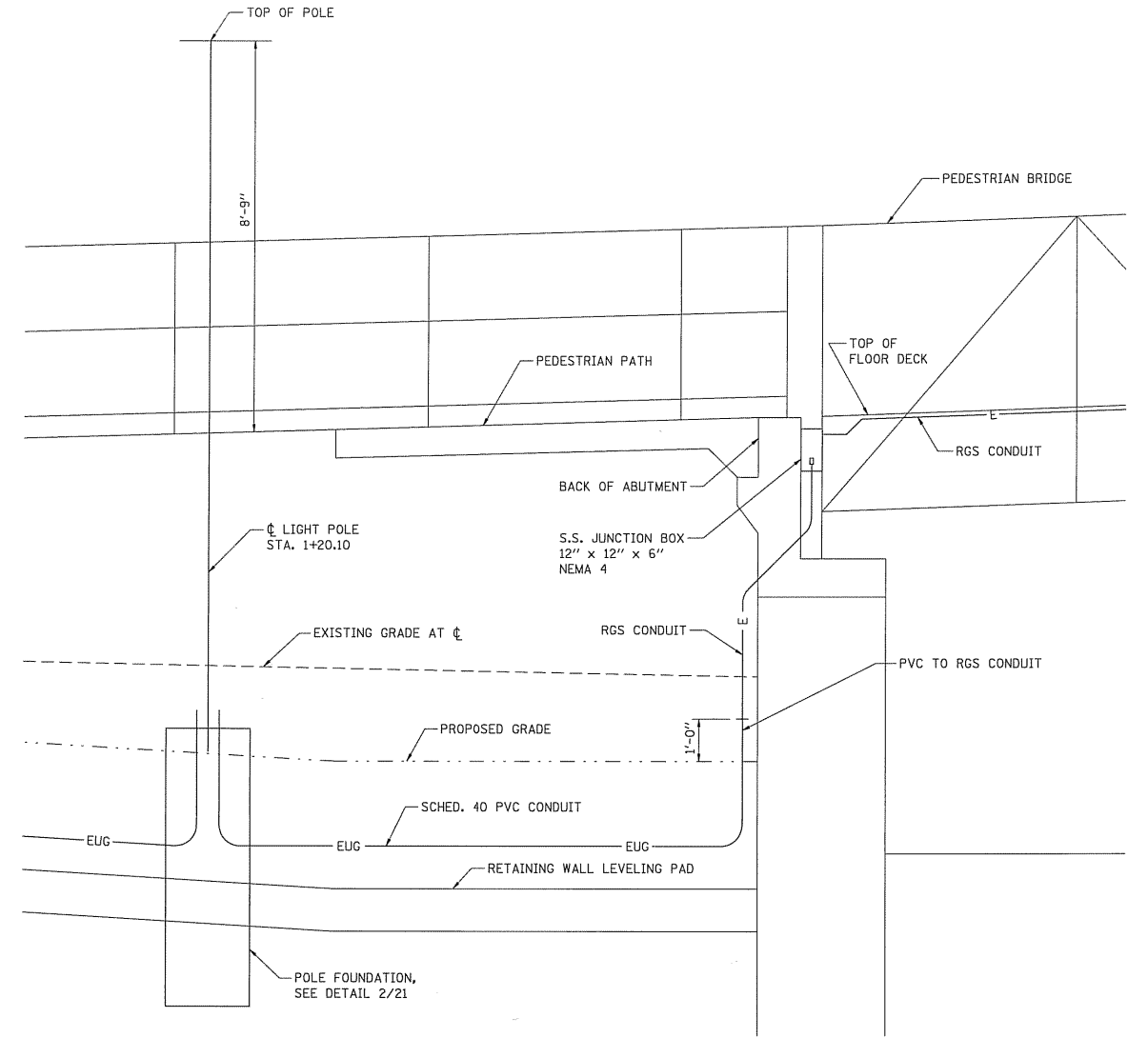
PEDESTRIAN PATH BRIDGE ABUTMENT ELEVATION SCALE: NONE
