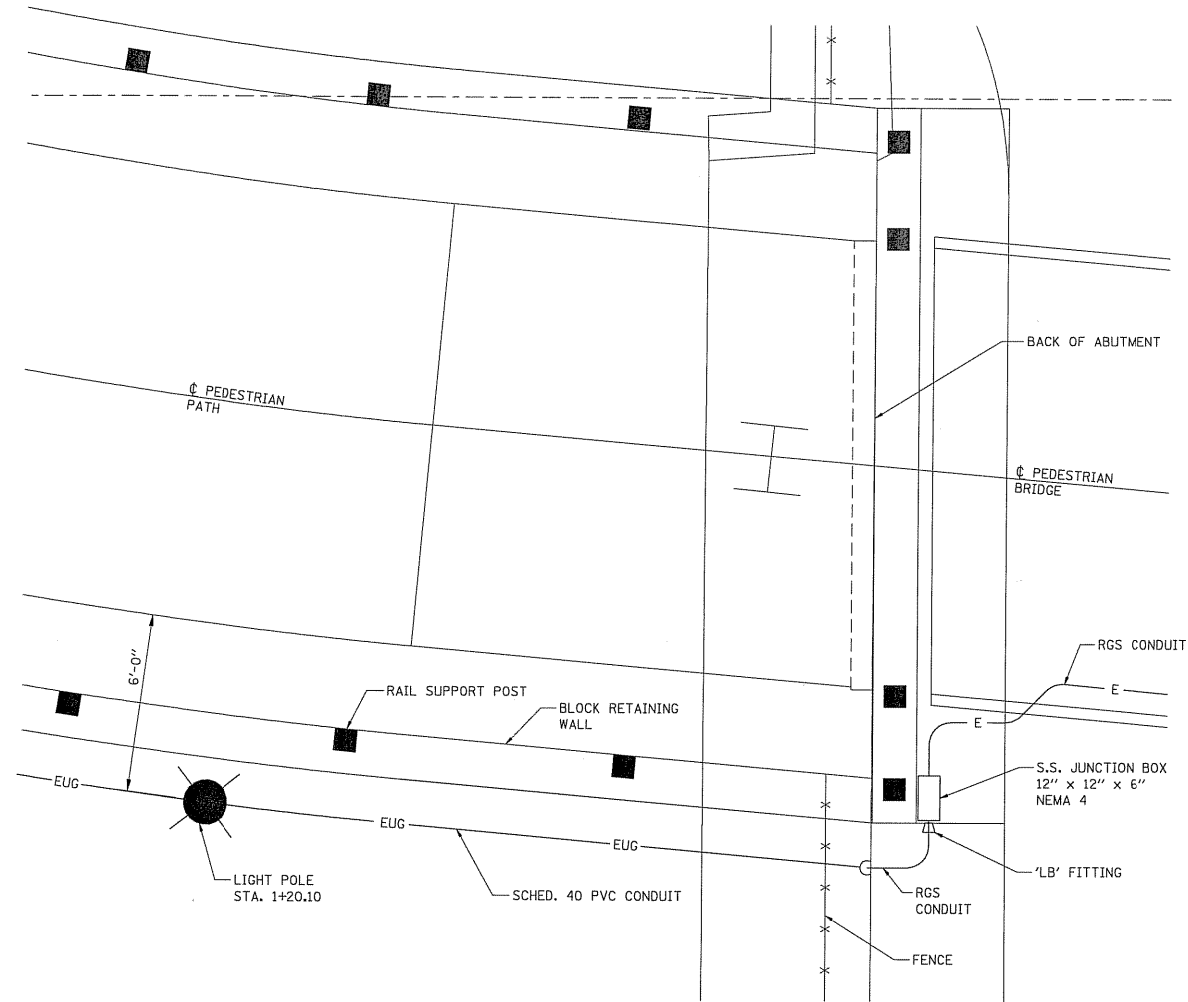
PEDESTRIAN PATH BRIDGE ABUTMENT PLAN SCALE: NONE
