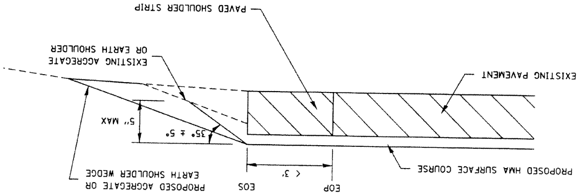
NO MILLING; ADJACENT SHOULDER FLUSH WITH OR LOWER THAN EXISTING PAVEMENT
