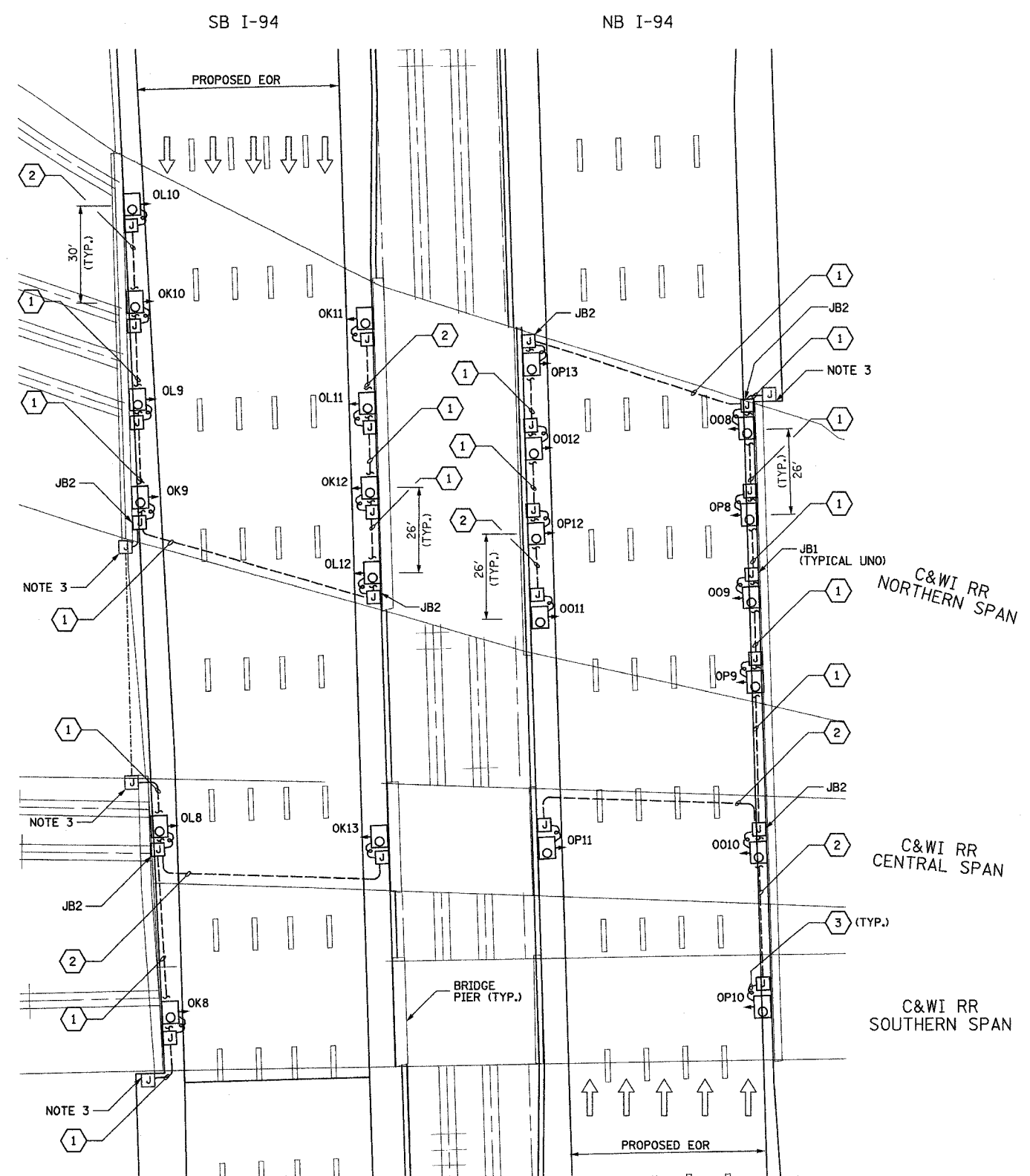
PROPOSED UNDERPASS LIGHTING PLAN
