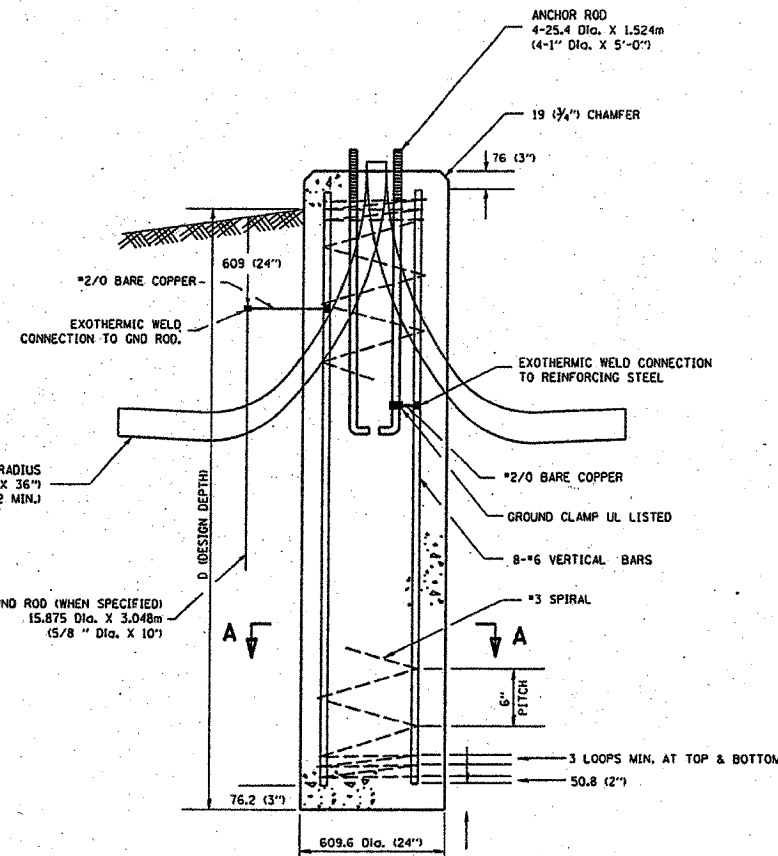
FOUNDATION DETAIL
