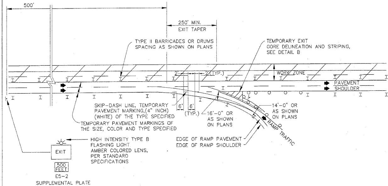
TYPICAL APPLICATION OF TEMPORARY EXIT GORE DELINEATION AND SIGNING
