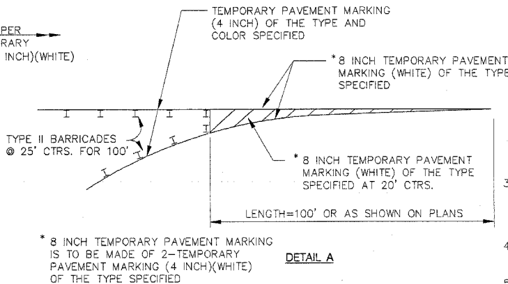
TEMPORARY ENTRANCE GORE STRIPING
