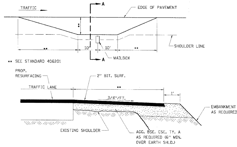
SECTION A-A MAILBOX TURNOUT DETAILS
