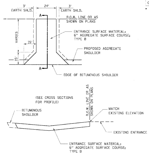
FIELD ENTRANCE DETAIL
