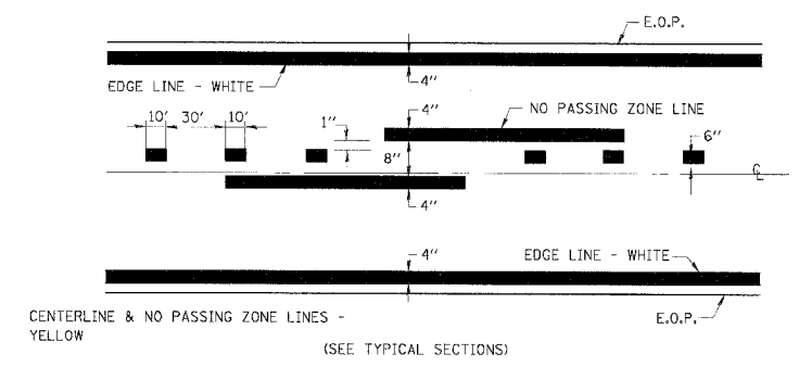
PAVEMENT MARKING DETAIL
