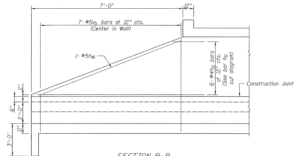
SECTION B-B (Floor reinforcement not shown)
