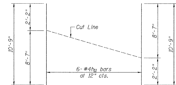
BAR h11 CUT DIAGRAM Order h11 bars full length. Layout in field according to diagram. Cut h11 bars along cut line. Use remainder of each bar in opposite wall.
