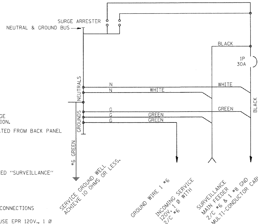
SCHEMATIC DIAGRAM
