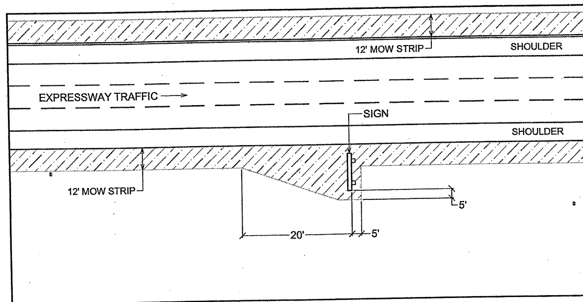
Mowing Detail #4
