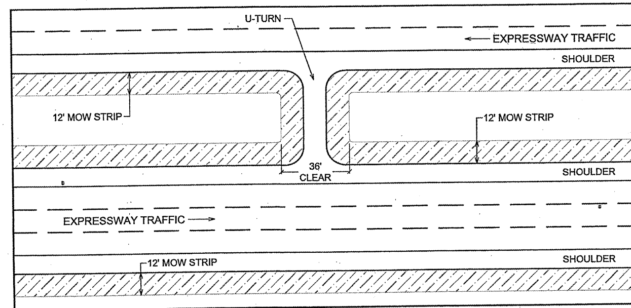
Mowing Detail #5
