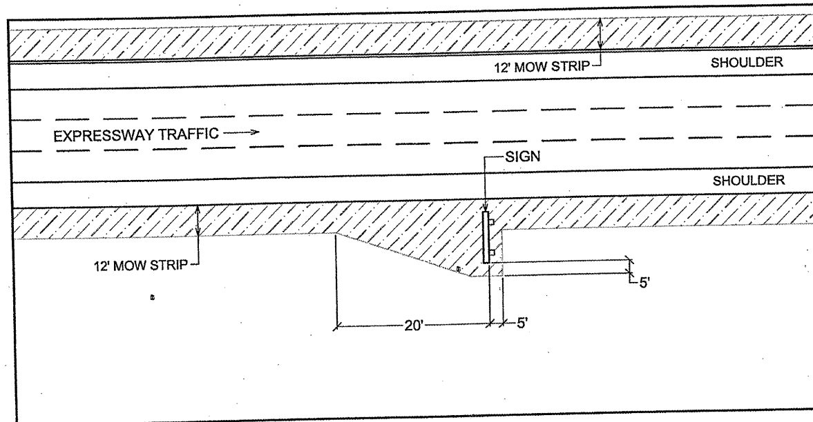
Mowing Detail #4 Roadway Signs
