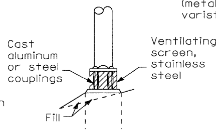
BREAKAWAY COUPLING
