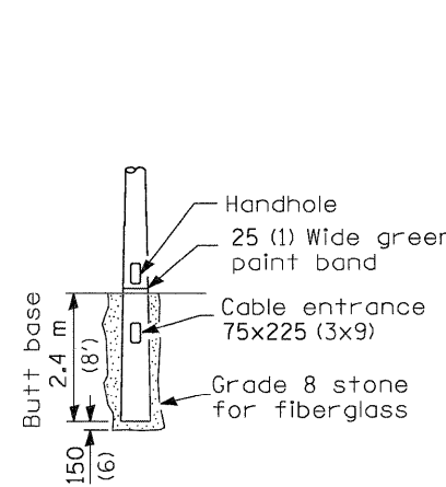
BUTT BASE
