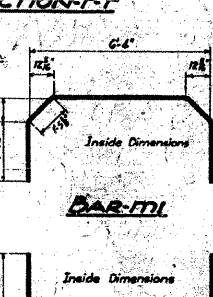
SECTION-F-F
