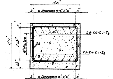
SECTION-H-H
