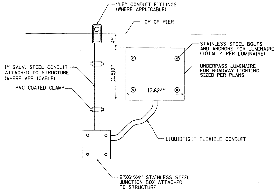
TYPICAL SURFACE MOUNTED UNDERPASS LUMINAIRE AND JUNCTION BOX MOUNTING DETAIL NOT TO SCALE
