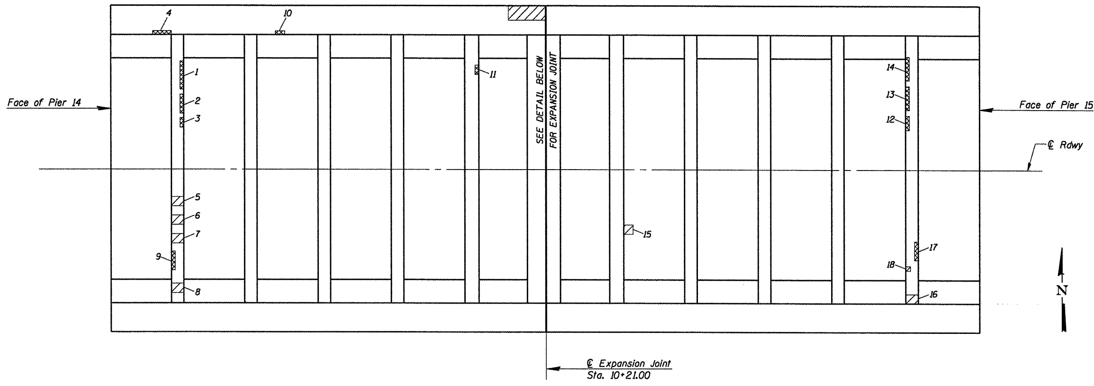
STRUCTURE REPAIR PLAN AT FLOOR BEAMS (Span 14)
