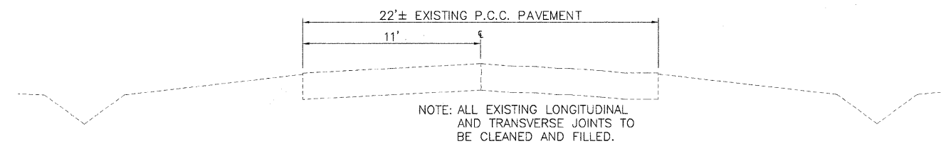
PROPOSED TYPICAL SECTION - A STA. 0+00 TO STA. 349+34.19 BACK=353+35.81 AHEAD
