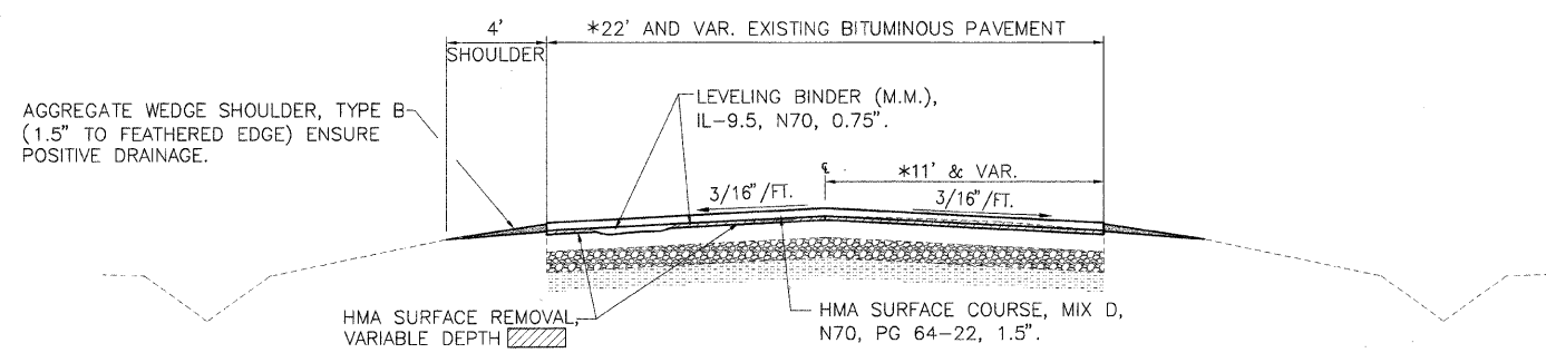
PROPOSED TYPICAL SECTION - B STA. 349+34.19 BACK=353+35.81 AHEAD TO STA. 418+23 BRIDGE OMISSION STA. 375+81.81 TO STA. 379+15.35 *VARIABLE WIDTH PER TRANSITION STA. 418+23 TO STA. 419+73
