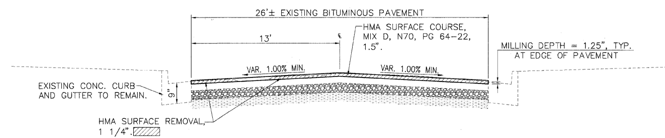
PROPOSED TYPICAL SECTION - C STA. 419+73 TO STA. 463+64.84
