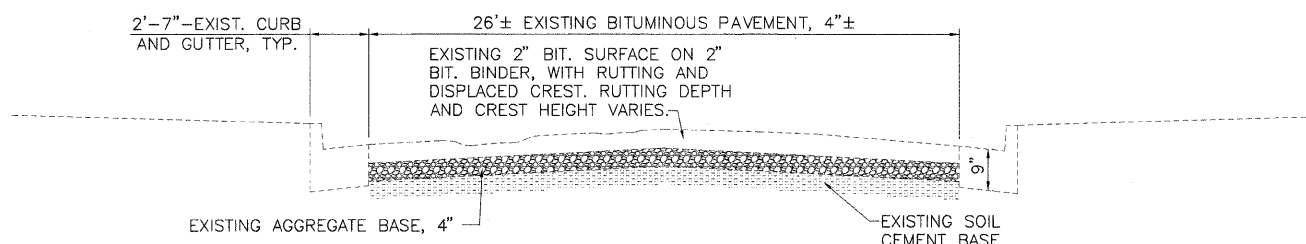
EXISTING BITUMINOUS PAVEMENT WITH CURB AND GUTTER STA. 419+73 TO STA. 463+64.84
