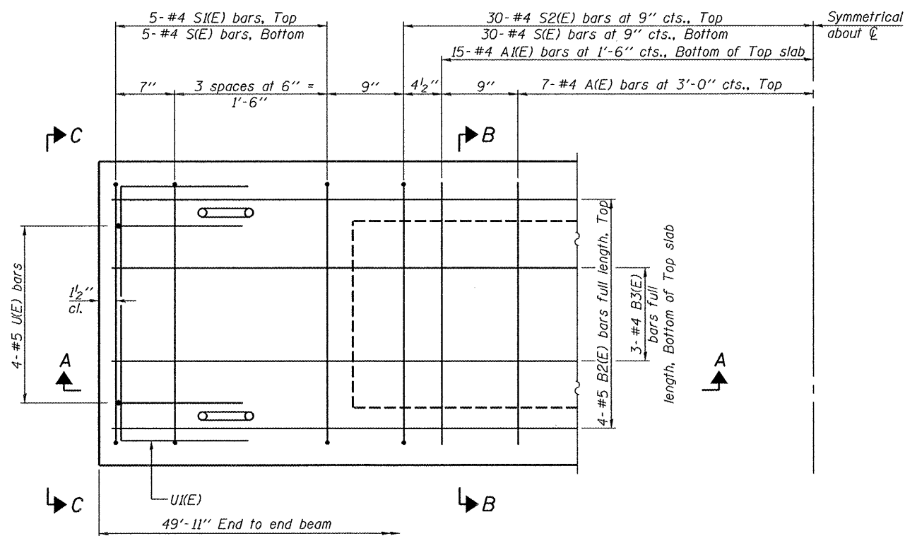
PLAN VIEW
