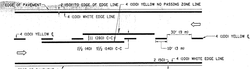
2-LANE ROADWAY
