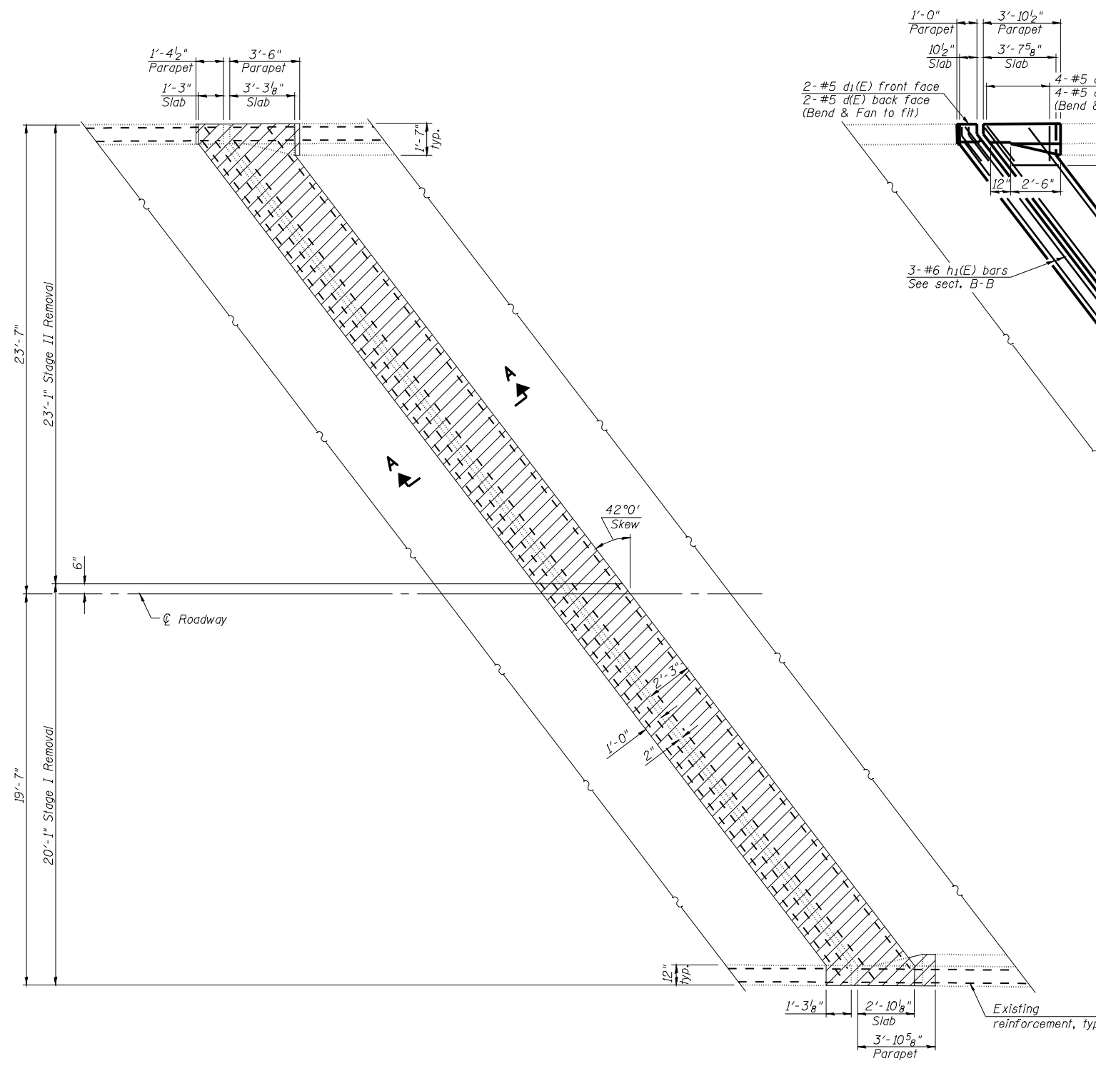
PARTIAL REMOVAL PLAN (South Abutment SN 001-0062)
