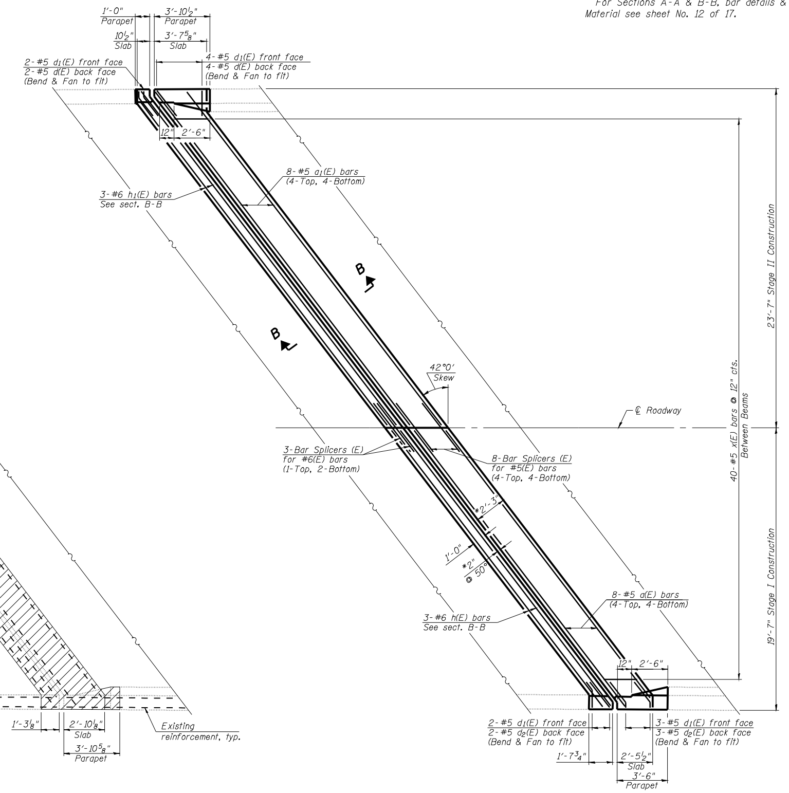
PARTIAL PROPOSED PLAN (South Abutment SN 001-0062)
