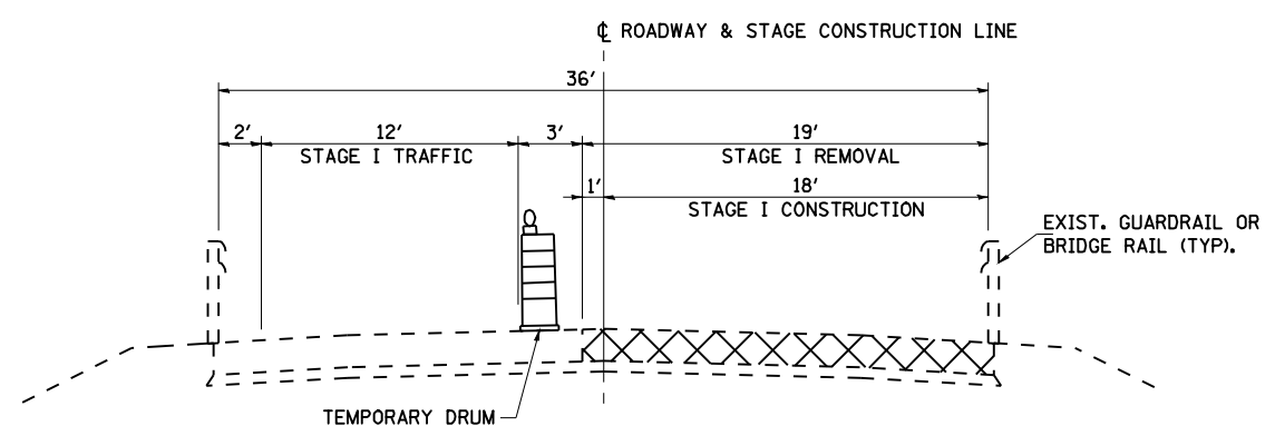
TYPICAL SECTION - STAGE I CONSTRUCTION
