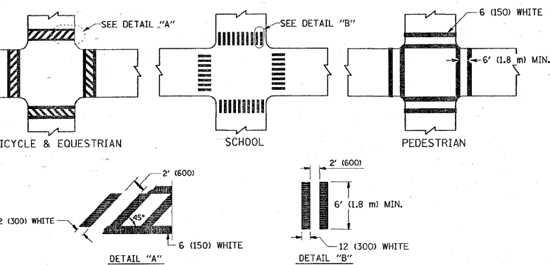
TYPICAL CROSSWALK MARKING
