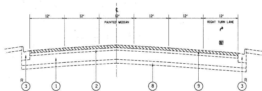
EXISTING TYPICAL CROSS SECTION STA. 75+93 TO 79+64
