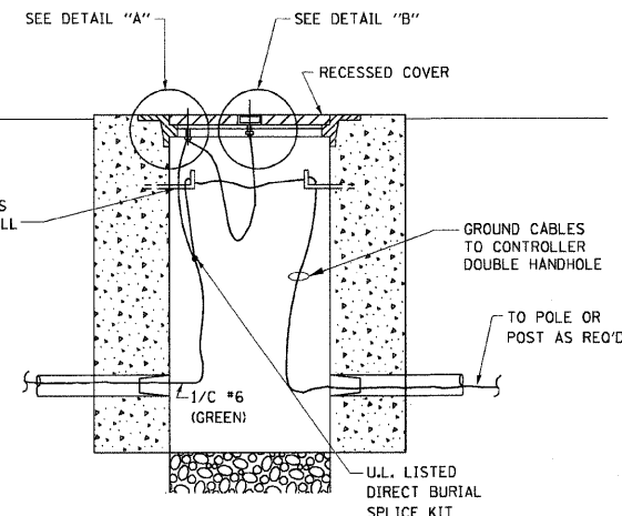
HANDHOLE COVER & FRAME - GROUNDING DETAIL
