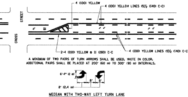
TYPICAL PAINTED MEDIAN MARKING
