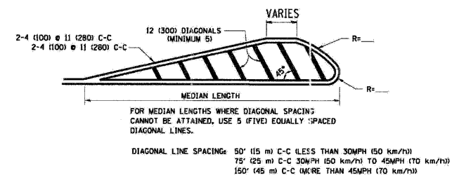
TYPICAL PAINTED MEDIAN MARKING
