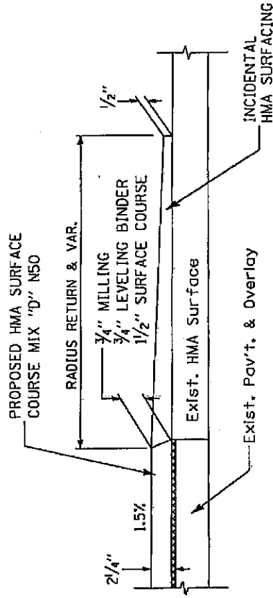
SIDEROAD & ENTRANCE DETAIL Not to Scale
