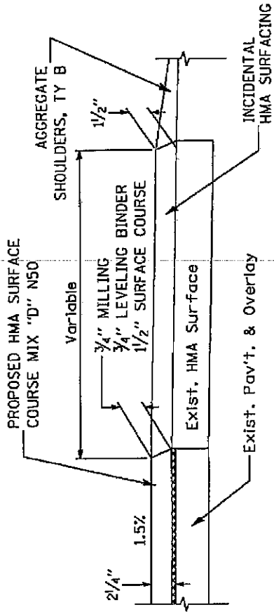
MAILBOX TURN OUT DETAIL Not to Scale
