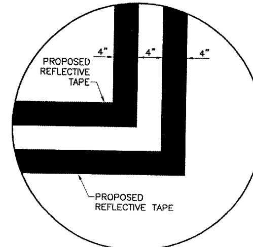
TEMPORARY MARKING DETAIL "NOT TO SCALE"
