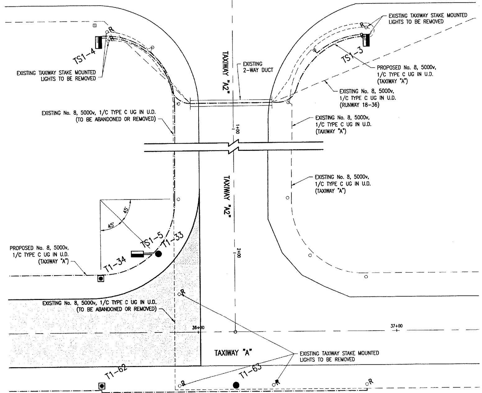
ENLARGED DETAIL OF TAXIWAY "A2" INTERSECTIONS NOT TO SCALE
