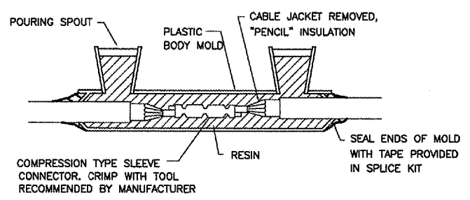
TYPE A - CABLE SPLICE
