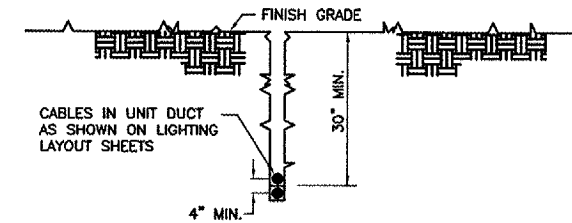
CABLE IN UNIT DUCT - PLOWED NOT TO SCALE
