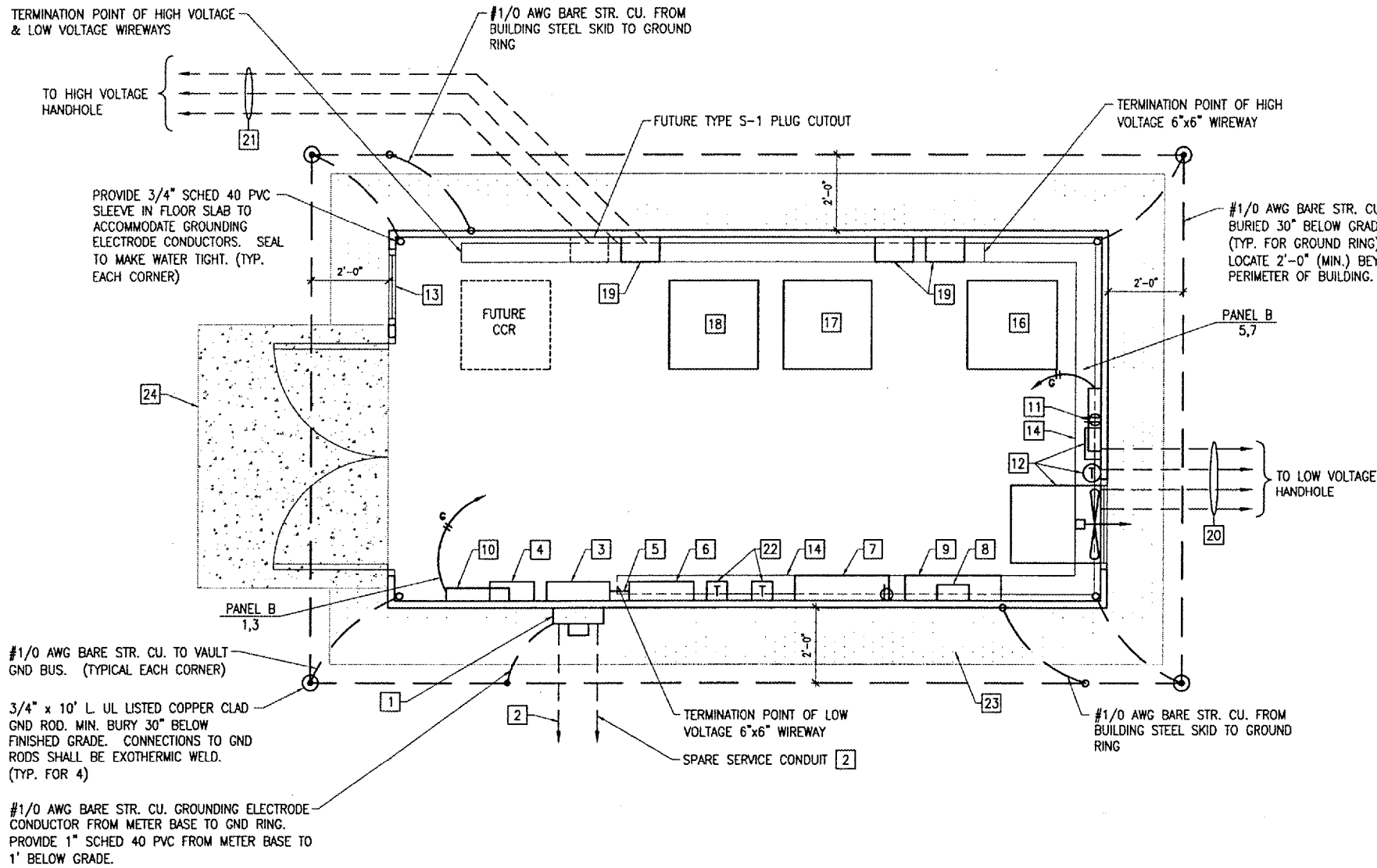
N VAULT ELECTRICAL EQUIPMENT PLAN SCALE 1/2"=1'-0" 1 0 2 4 FEET
