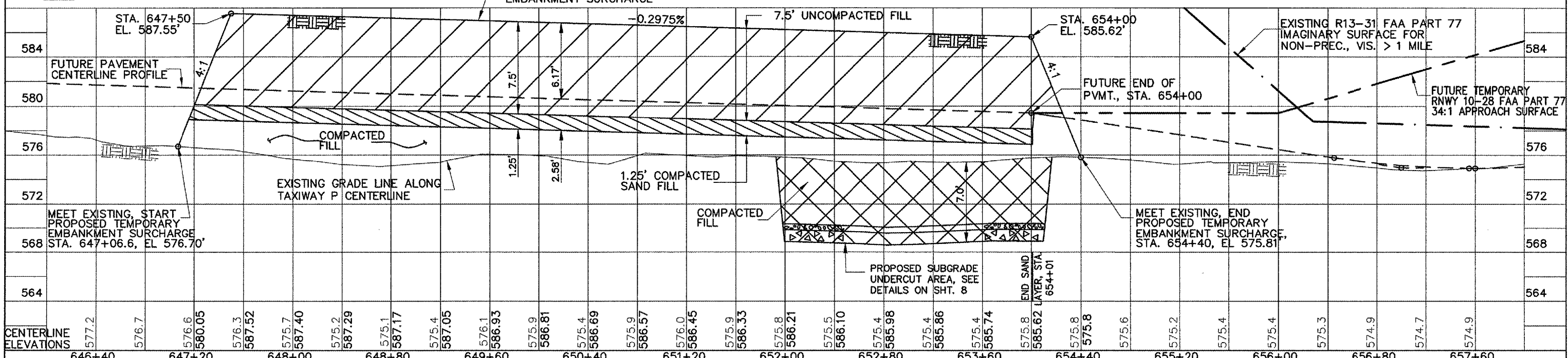
TAXIWAY P PLAN & PROFILE, STA 646+60 TO STA 657+40
